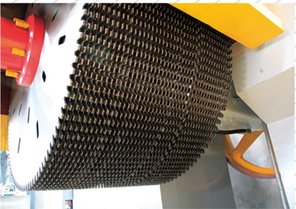
下刀量采用旋转编码器检测，精度高，同时可任意设定上、下行程位置，减小人员劳动强度。 Feeding depth is measured by Rotay Encoder to ensure its High-precision,meanwhile,upper and lower rtaveling distance can be set to reduce the labor intensity kf worker.
